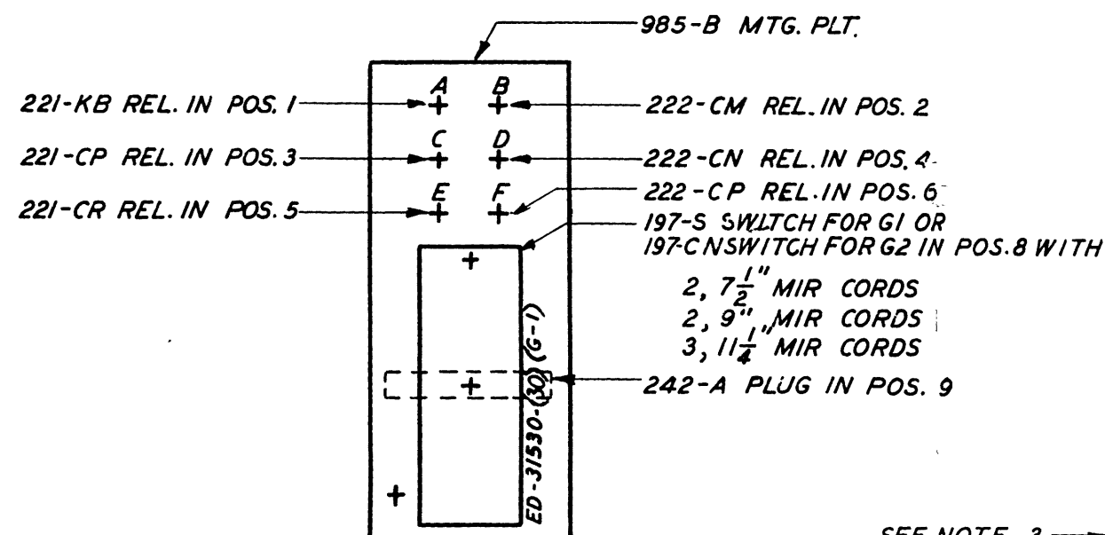
MOUNTING PLATE EQUIPMENT FIG. 1
